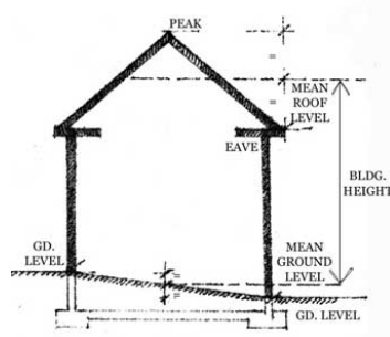
Figure 2-2: Building Height
