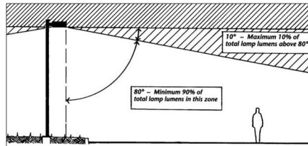
Figure 2-7: Full Cut-Off
