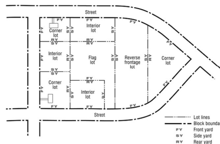
Figure 16-1: Lots
