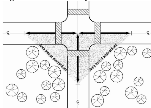
Figure 16-3: Visibility at Intersections
