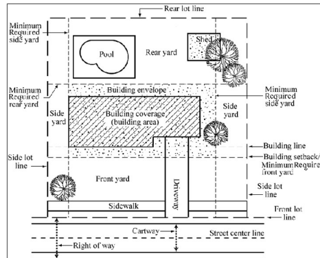
Figure 2-19: Yard Requirements
