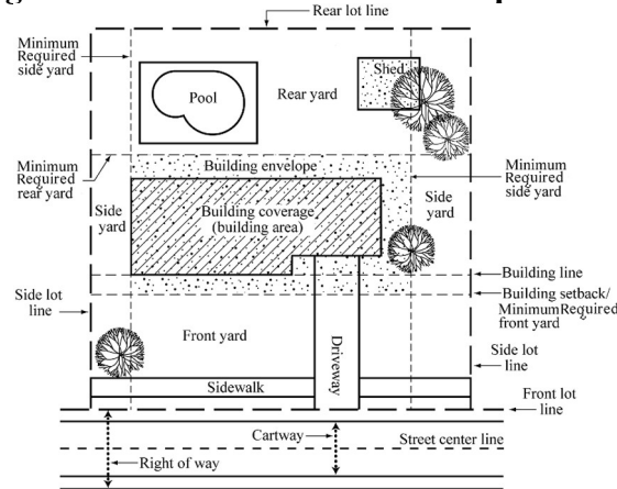
Figure 16-2: Yard and Setback Requirements
