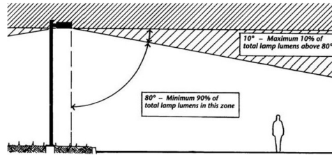
Figure 16-5: Full-Cutoff Lighting
