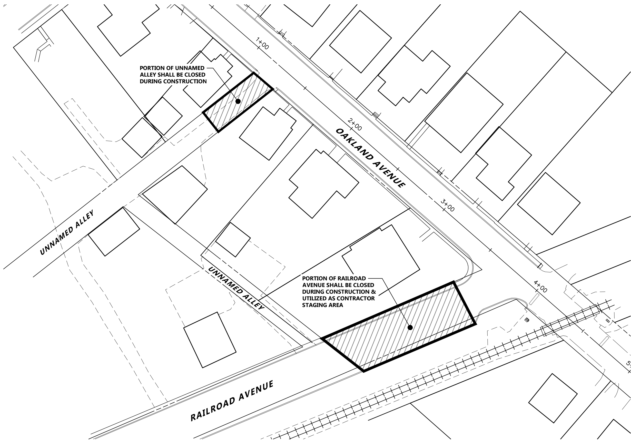
CONTRACTOR STAGING & ROAD CLOSURE PLAN SCALE: 1" = 40'
